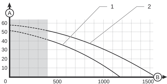
Vízhozam görbe : THEMA CONDENS F AS 30
