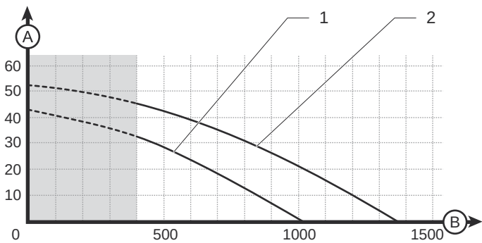
Vízhozam görbe : THEMA CONDENS F AS 25
