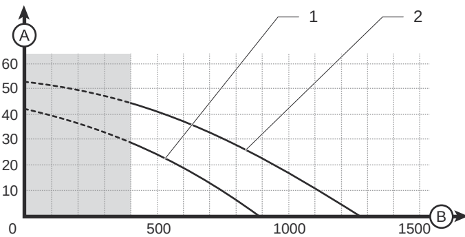
Vízhozam görbe : THEMA CONDENS F AS 12 + F 25
